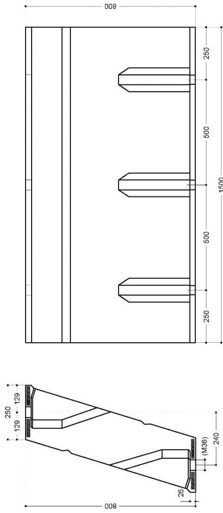
RUBBER FENDER PLAN DRAWING SIZE: 800H X 1500L
