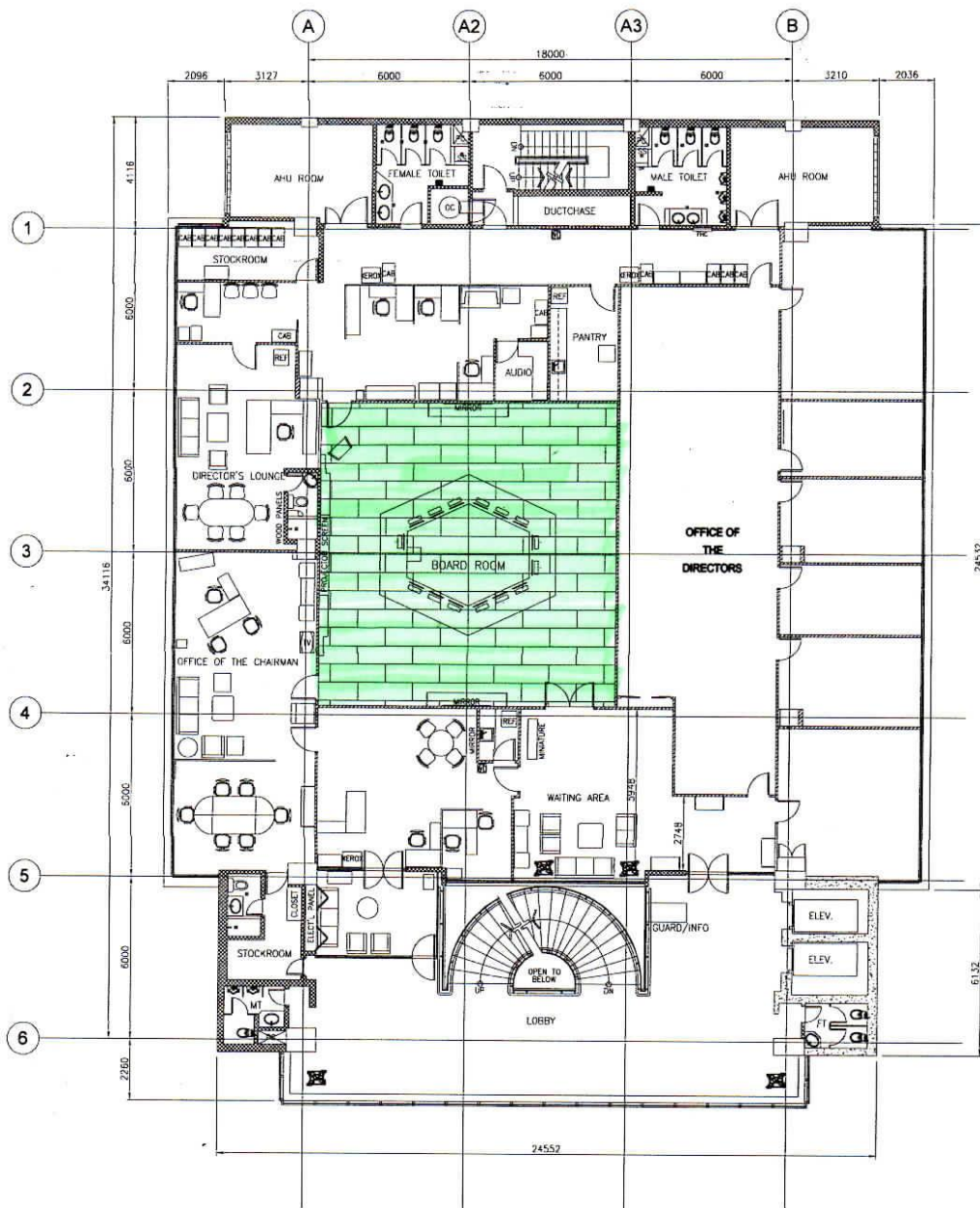
2 5TH FLOOR PLAN A-03 SCALE 1:100M
